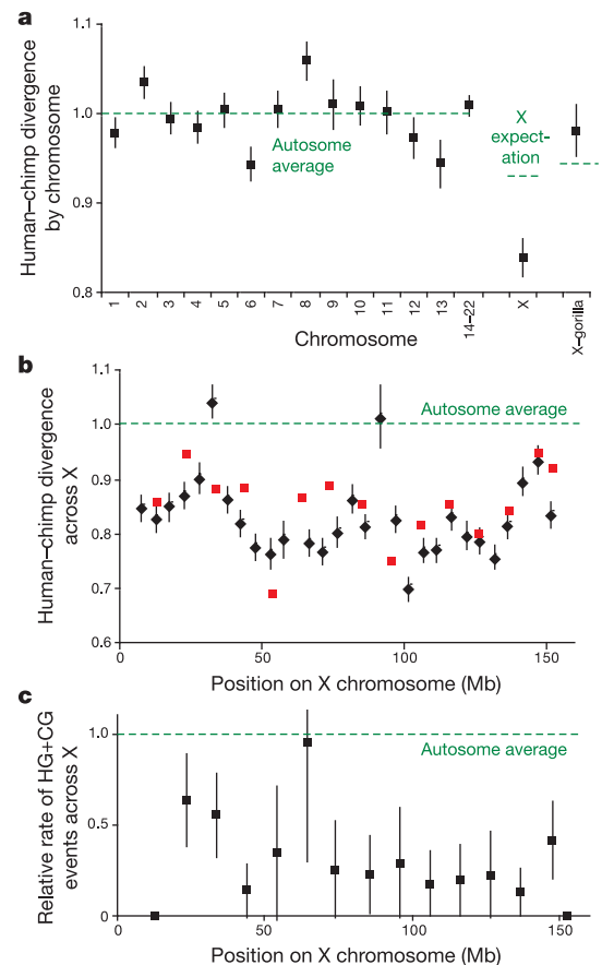
Figure 3 | Reduced human–chimpanzee time divergence across chromosome X. a , Human–chimpanzee genetic divergence is lower on chromosome X than on every other chromosome (HCGOM shotgun data, correcting for recurrent mutation), and lower than the theoretical expectation of about 93% for a constant-sized, freely mixing ancestral population (Supplementary Note 5). By contrast, the gorilla chromosome X comparison shows no decrease beyond the expectation of about 95% from theory. We have included a category pooling all chromosomes of less than 100 Mb in size, because the smaller chromosomes do not have much data and thus have large standard errors. b , The low time divergence is seen along nearly the entire X chromosome. Black symbols show the ratio of human–chimpanzee to human–macaque divergence plotted in non-overlapping 5-Mb bins in the 15.1 Mb of HCOM alignment. For comparison we also show the ratio of human–chimpanzee to human–gorilla divergence (10-Mb bins) in 372 kb of HCGOM shotgun data (red, \pm 1 standard error bars removed for clarity). c , The rate of HG and CG sites (HCGOM shotgun data, 10-Mb bins) is also greatly reduced along chromosome X, which is consistent with humans and chimpanzees being most closely related essentially everywhere along chromosome X.
